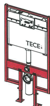
INWALL CISTERN FULLY FRAMED SLIMLINE 90MM WELS 4 STAR 9.300.057
