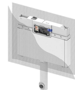
INWALL CISTERN SLIMLINE 90MM WELS 4 STAR 9.370.057
